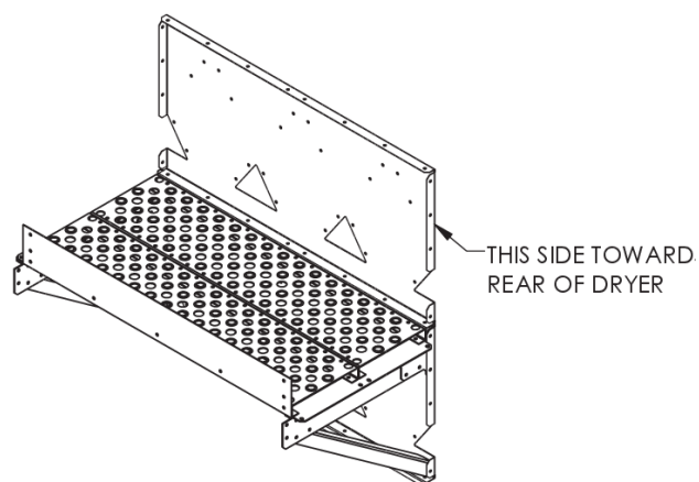
Fig. 11 – Attaching planks
