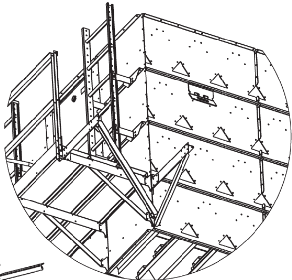
Fig. 9 – Attaching back right corner bracket
