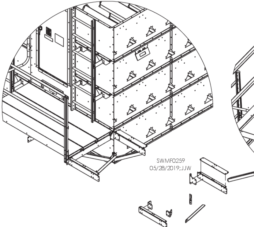
Fig. 9 – Attaching back right corner bracket
