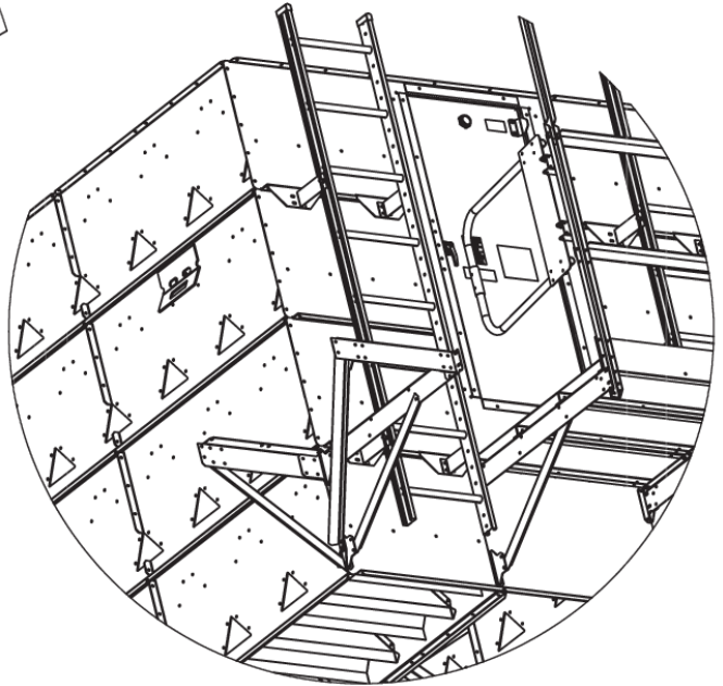
Fig. 8 – Attaching back left corner bracket
