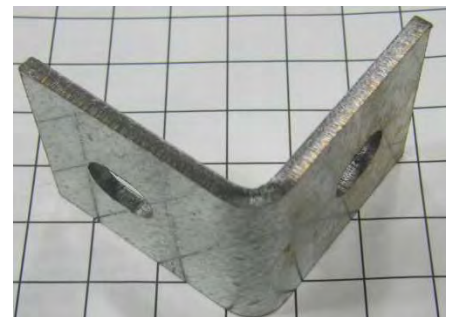
BT54519 – CORNER SPLICE PLATE FOR SUPPORT TOWER PLATFORM
