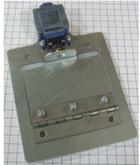
Y6595 – PRESSURE RELIEF DOOR ASSY. FOR DOUBLE-RUN HEAD SECTION
