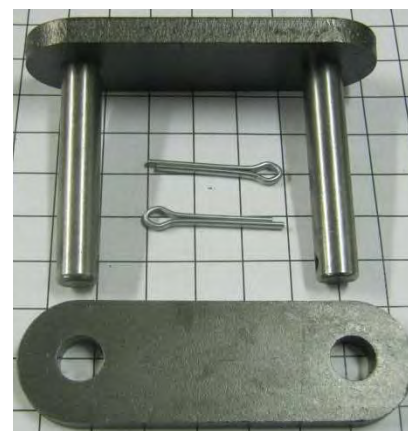
J1793 – CONNECTOR LINK, D81XHH CHAIN, W/ COTTER PIN J1794
