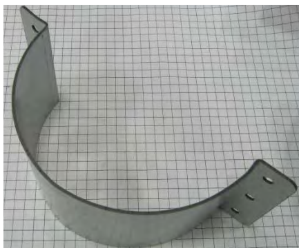
Y7041 – HALF BAND TUBE CLAMP, 10" DOUBLE RUN
